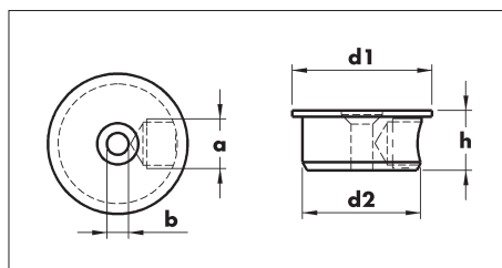
Pot-Shaped Staircase Conn.
