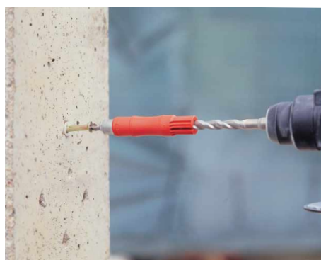
Set and screw in the anchor.
